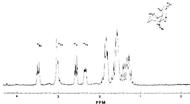
Figure 2. NMR spectrum (300 MHz) of (4 \alpha ,5 \beta ,8 \alpha )-decahydroquinoline-5-carboxylic acid ( cis -2).
