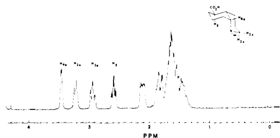
Figure 1. NMR spectrum (300 MHz) of (4 \alpha ,5 \alpha ,8 \alpha )-decahydroquinoline-5-carboxylic acid ( cis -1).
