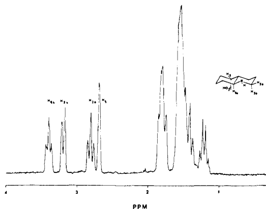
Figure 3. NMR spectrum (300 MHz) of (4 \alpha ,5 \beta ,8 \alpha\beta )-decahydroquinoline-5-carboxylic acid ( trans - 3 ).
