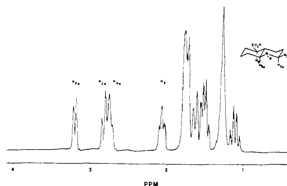
Figure 4. NMR spectrum (300 MHz) of (4 \alpha ,5 \alpha ,8 \alpha\beta )-decahydroquinoline-5-carboxylic acid ( trans - 4 ).
